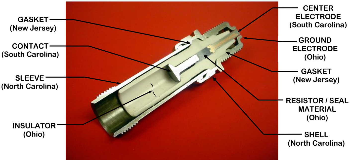
TEMPEST ® MASSIVE ELECTRODE SPARK PLUG
