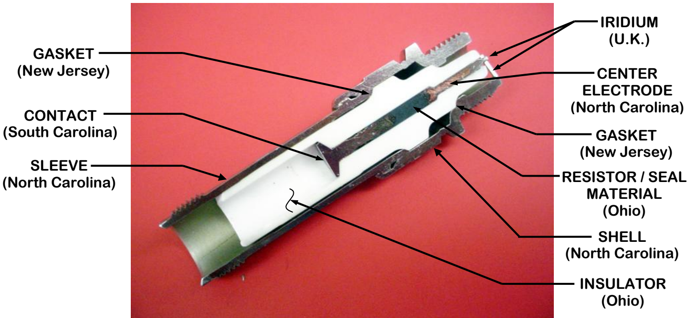
TEMPEST ® FINE WIRE ELECTRODE SPARK PLUG
