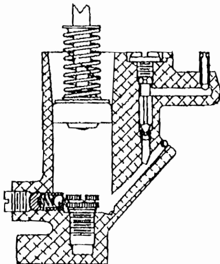
OLD STYLE (36-539) KNURLED HEAD USED WITH BALL SAFETY RATCHET
